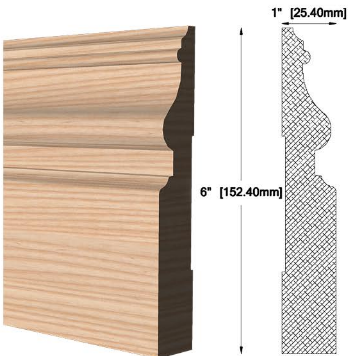
PL-6018 1" X 6" (25.40 X 152.40 mm)
