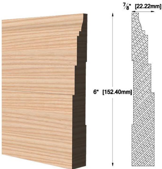
PL-6038 7/8" X 6" (22.22 X 152.40 mm)
