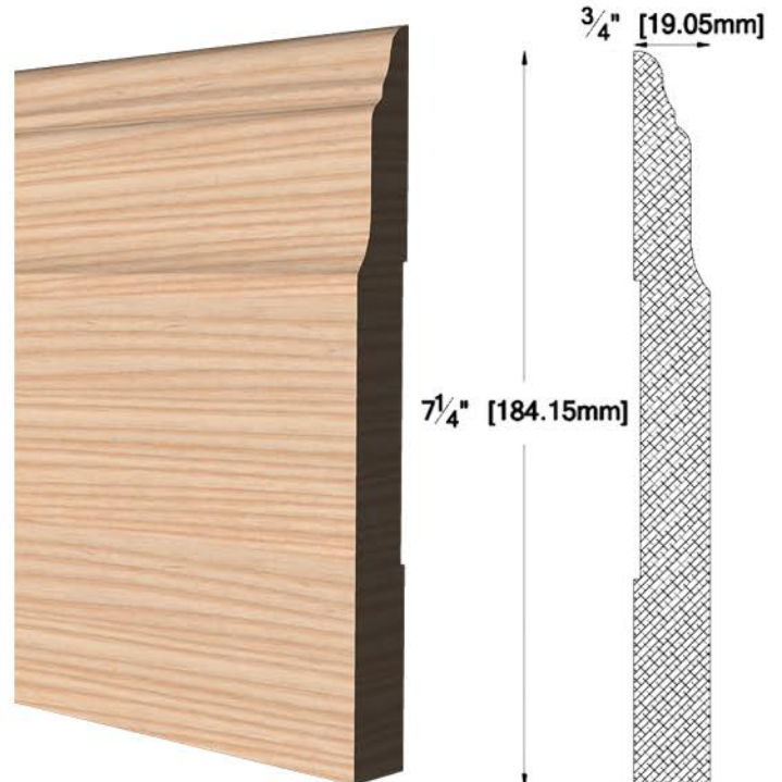
PL-7037 3/4" X 7 1/4" (19.05 X 184.15 mm)
