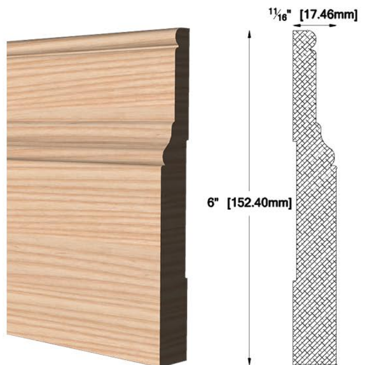
PL-6021 11/16" X 6" (17.46 X 152.40 mm)
