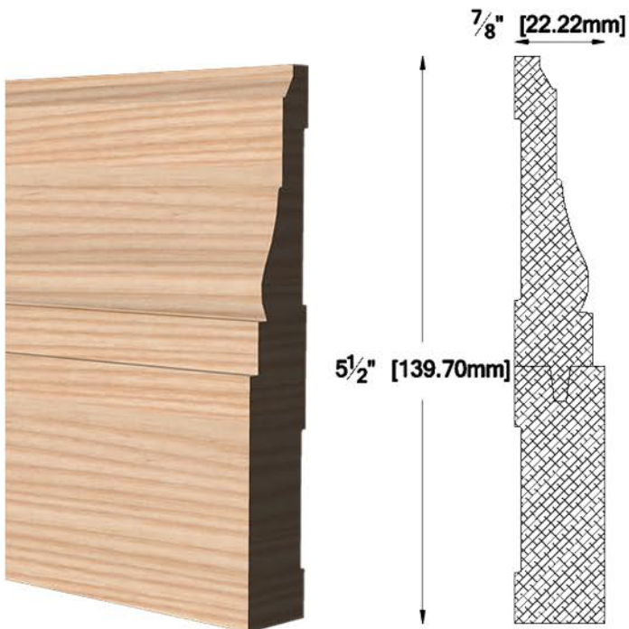
PL-5021 7/8" X 5 1/2" (22.22 X 139.70 mm)
