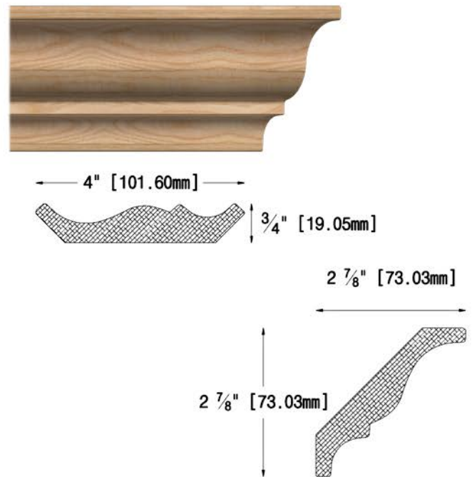
OG-4100 3/4" X 4" (19.05 X 101.60 mm)
