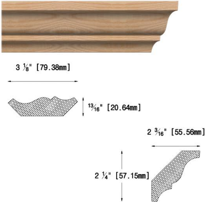
OG-3103 13/16" X 3 1/8" (20.64 X 79.38 mm)
