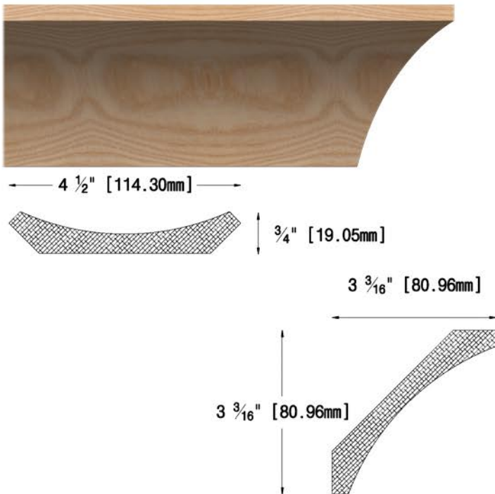
OG-4012 3/4" X 4 1/2" (19.05 X 114.30 mm)
