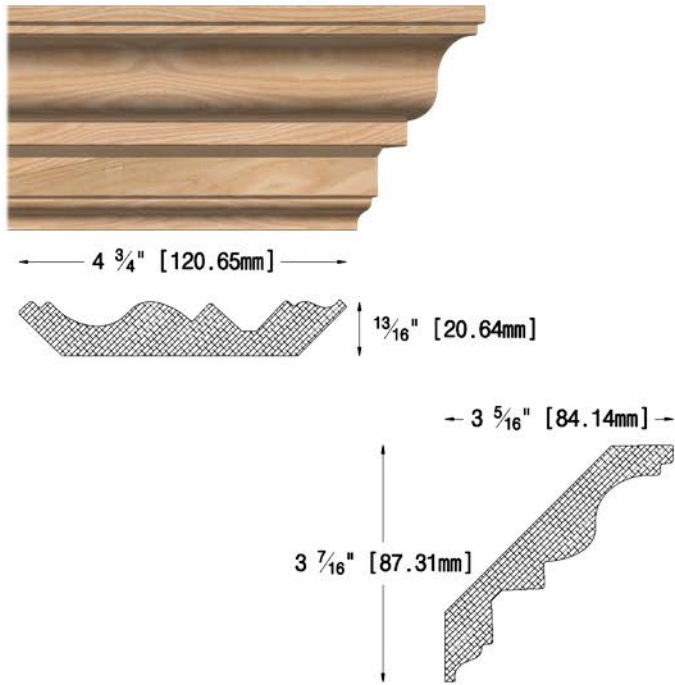
OG-4018 13/16" X 4 3/4" (20.64 X 120.65 mm)
