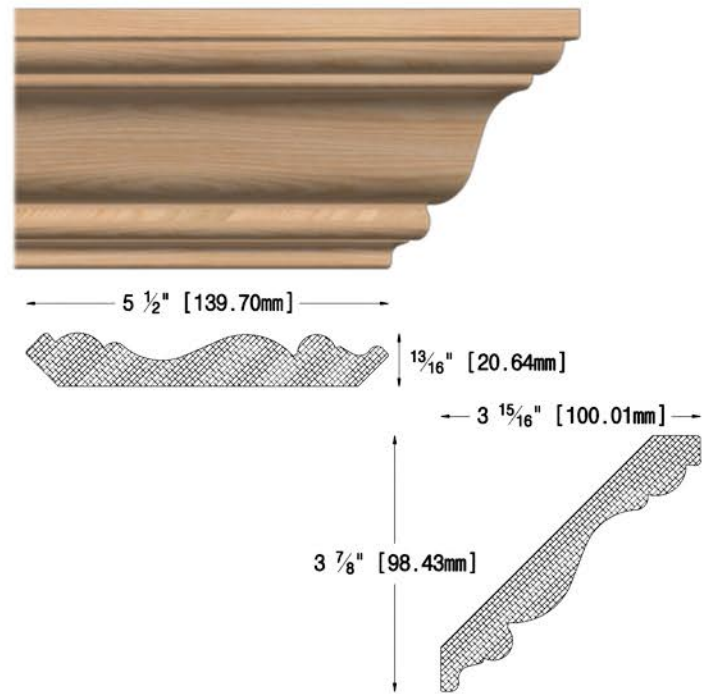
OG-5104 13/16" X 5 1/2" (20.64 X 139.70 mm)
