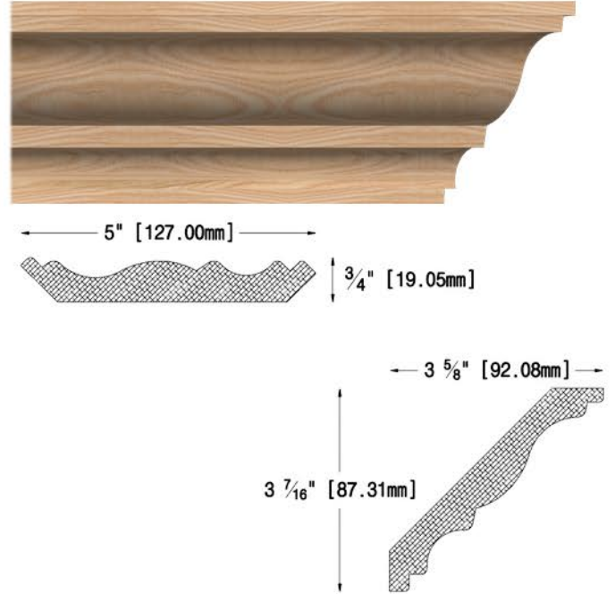
OG-5023 3/4" X 5" (19.05 X 127.00 mm)
