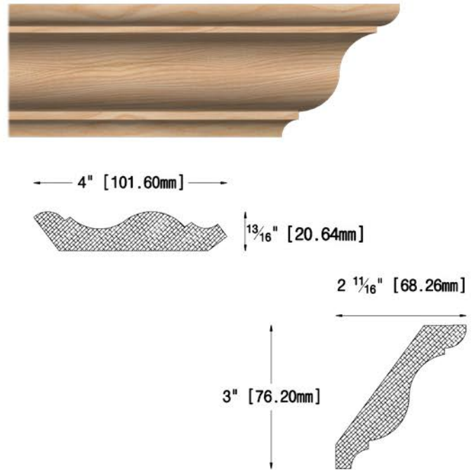
OG-4024 13/16" X 4" (20.64 X 101.60 mm)
