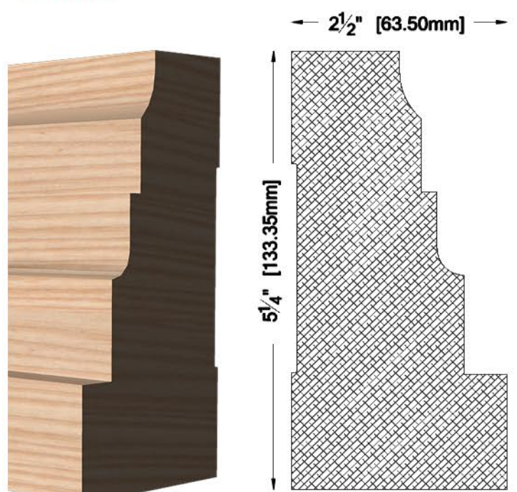
CA-5013 2 1/2" X 5 1/4" (63.50 X 133.35 mm)
