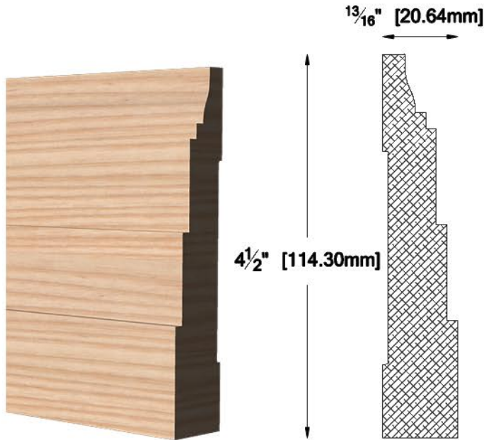
CA-3038 13/16" X 4 1/2" (20.64 X 114.30 mm)
