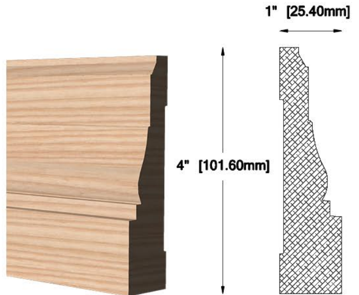
CA-4022 1" X 4" (25.40 X 101.60 mm)
