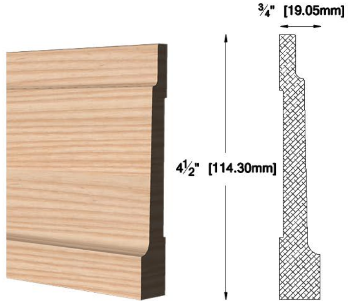
CA-3022 3/4" X 4 1/2" (19.05 X 114.30 mm)
