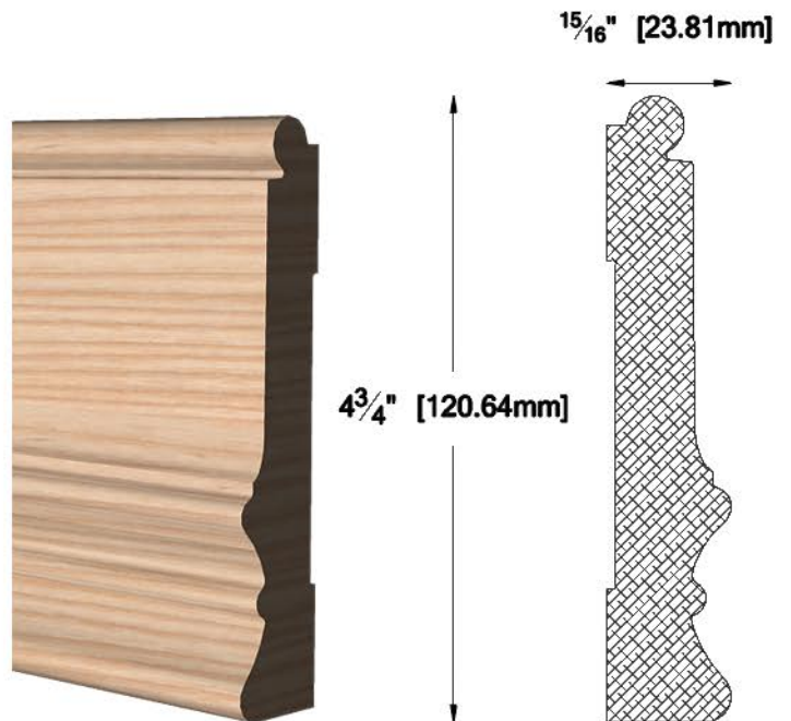
CA-4027 15/16" X 4 3/4" (23.81 X 120.64 mm)
