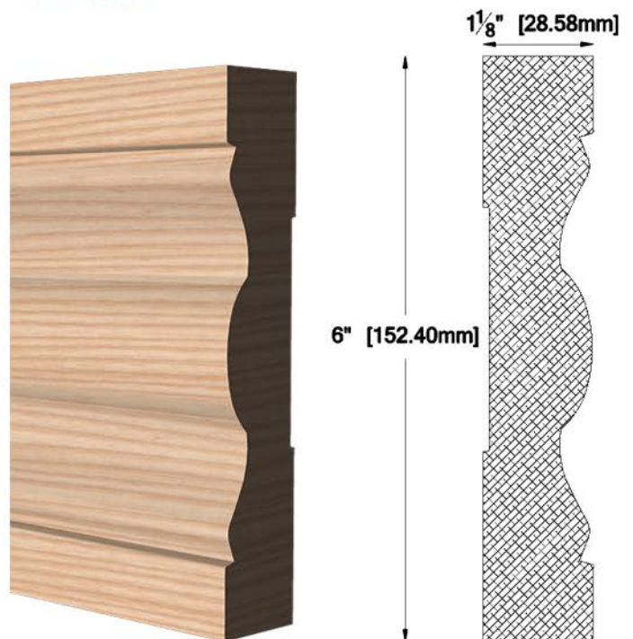
CA-6020 1 1/8" X 6" (28.58 X 152.40 mm)
