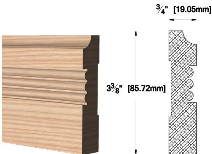
CA-3023 3/4" X 3 3/8" (19.05 X 85.72 mm)
