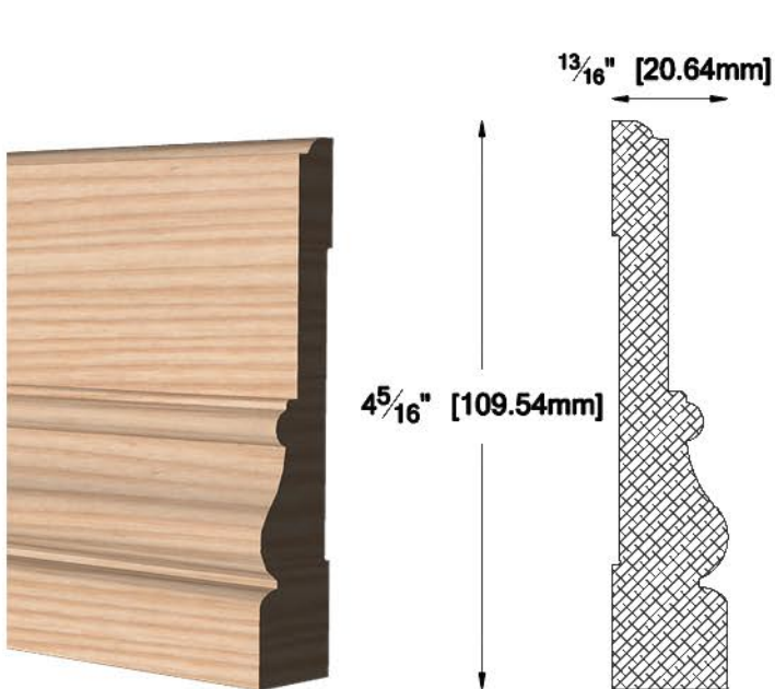
CA-4026 13/16" X 4 5/16" (20.64 X 109.54 mm)
