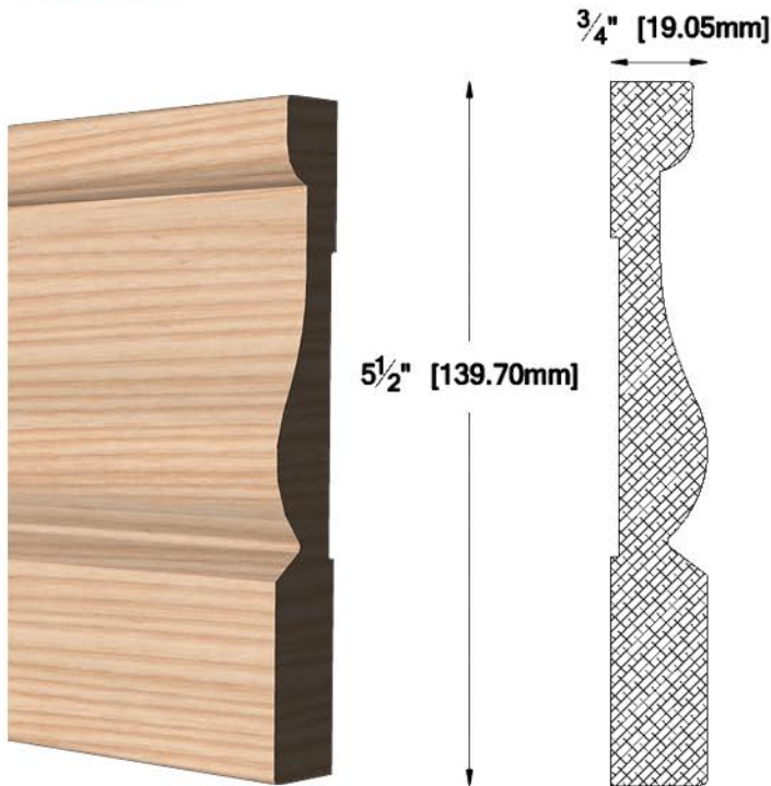
CA-5012 3/4" X 5 1/2" (19.05 X 139.70 mm)
