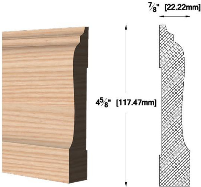
CA-4020 7/8" X 4 5/8" (22.22 X 117.47 mm)
