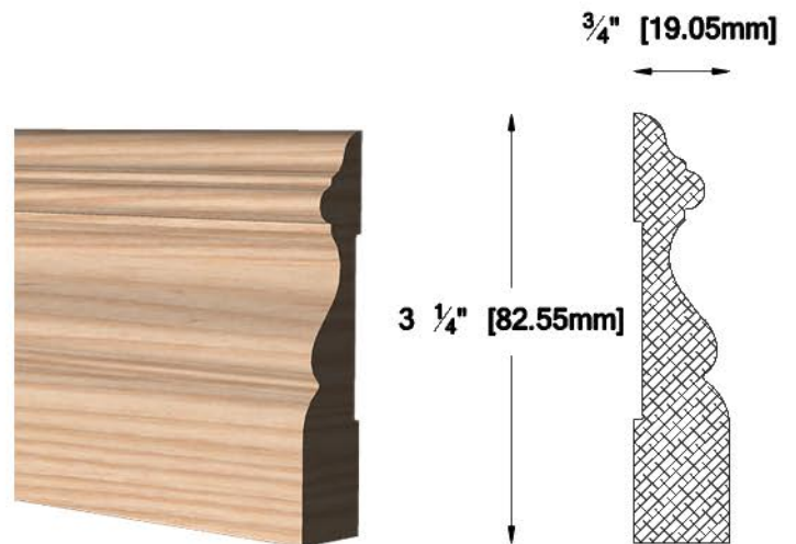
CA-3500 3/4" X 3 1/4" (19.05 X 82.55 mm)
